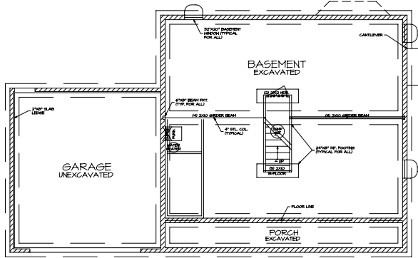
FOUNDATION PLAN A-3 SCALE: 1/4"=1'-0"
