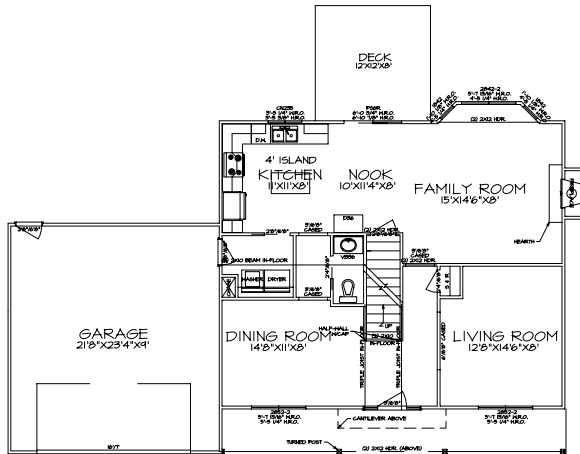
FIRST FLOOR PLAN A-4 SCALE: 1/4"=1'-0"
